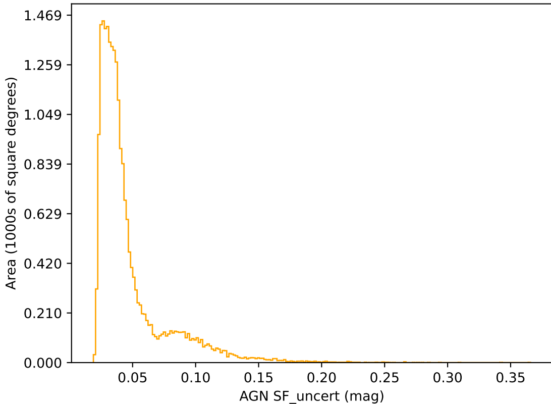
roll_3_v3.4_10yrs r band: AGN SF_uncert
