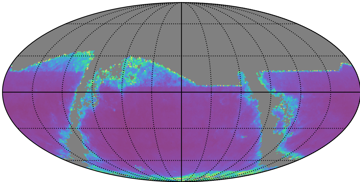
roll_3_v3.4_10yrs i band: AGN SF_uncert
