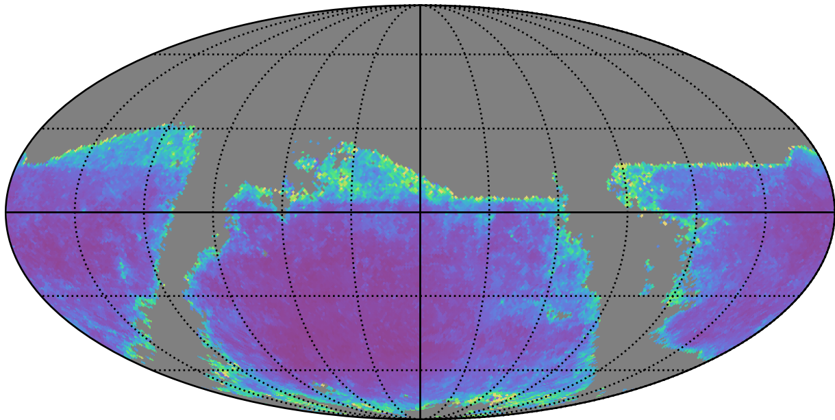
roll_3_v3.4_10yrs g band: AGN SF_uncert
