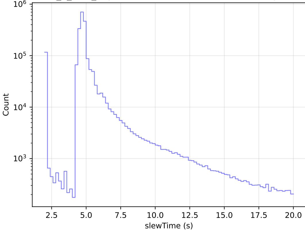
roll_3_v3.4_10yrs All visits: Zoom Slew Time Histogram
