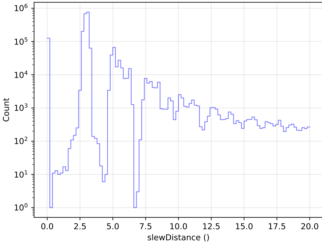
roll_3_v3.4_10yrs All visits: Zoom Slew Distance Histogram
