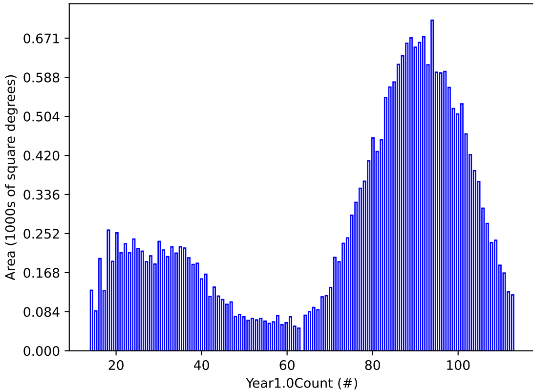
roll_3_v3.4_10yrs night &lt; 365.25: Year1.0Count
