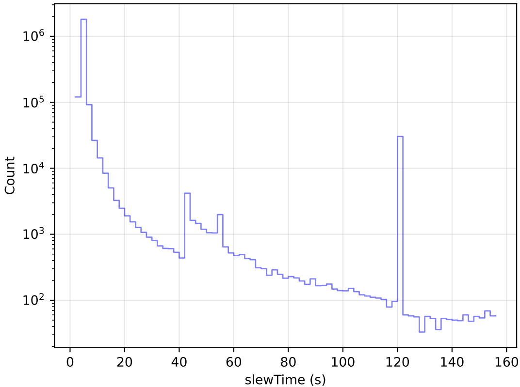
roll_3_v3.4_10yrs All visits: Slew Time Histogram
