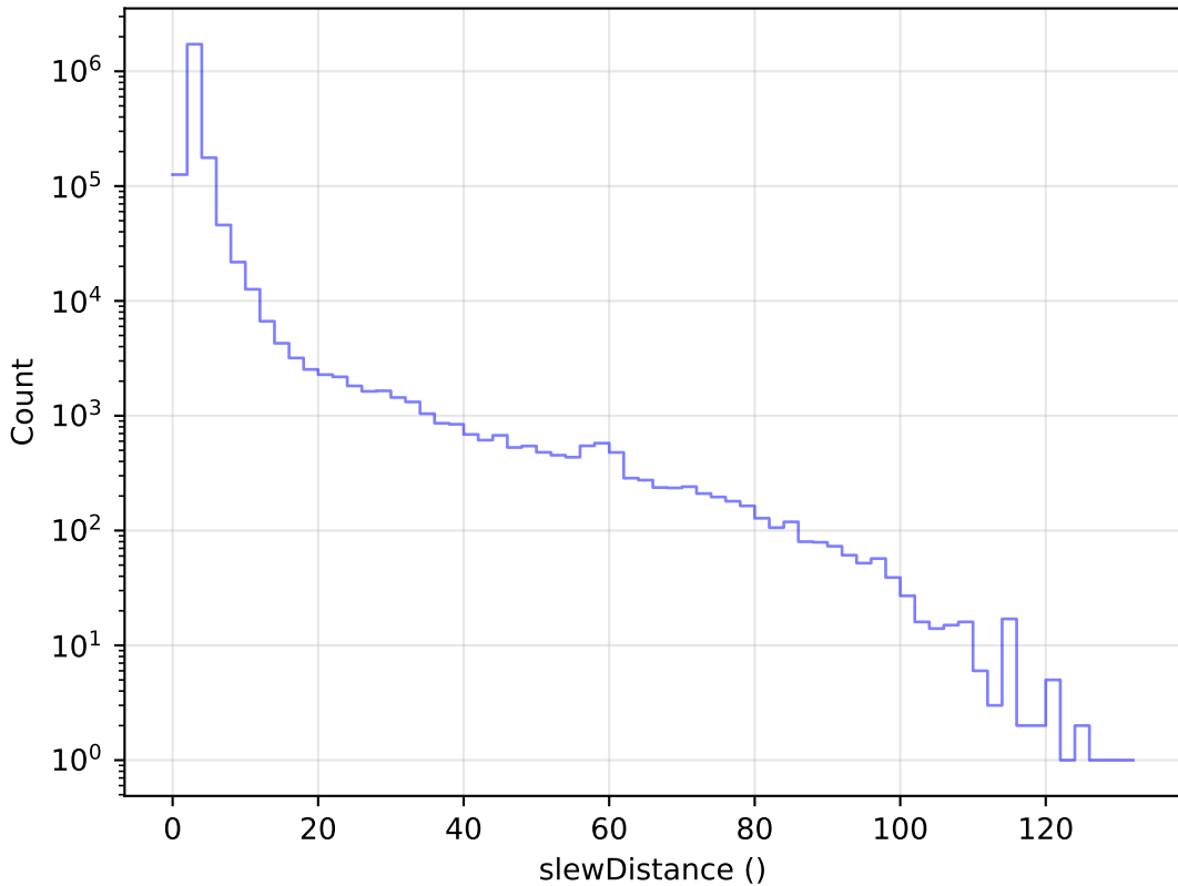
roll_3_v3.4_10yrs All visits: Slew Distance Histogram
