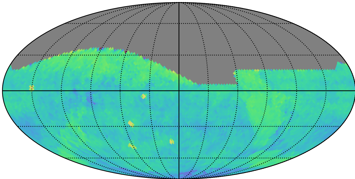
roll_3_v3.4_10yrs (g or r or i): PairFraction
