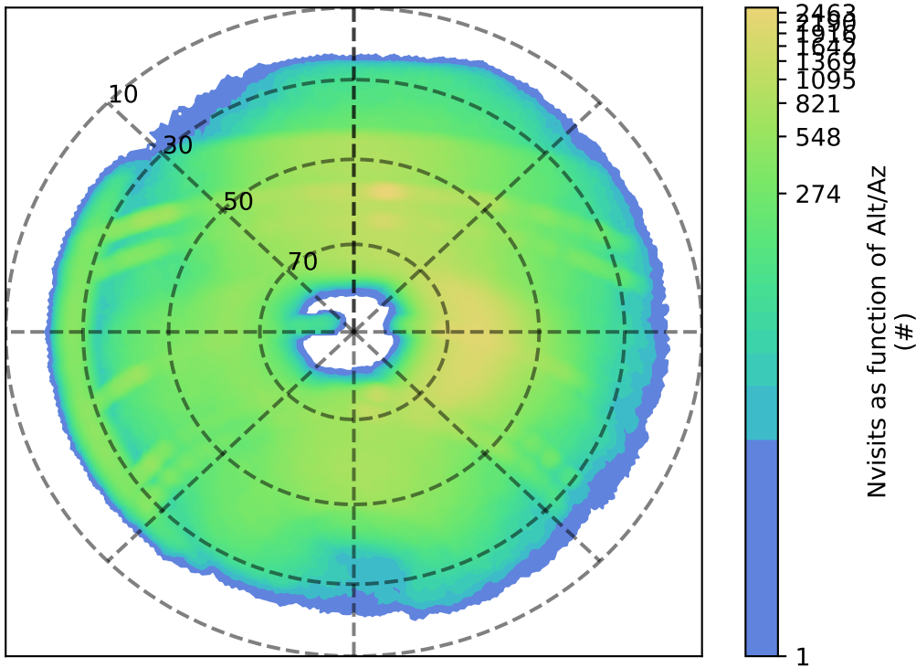
roll_3_v3.4_10yrs r: Nvisits as function of Alt/Az
