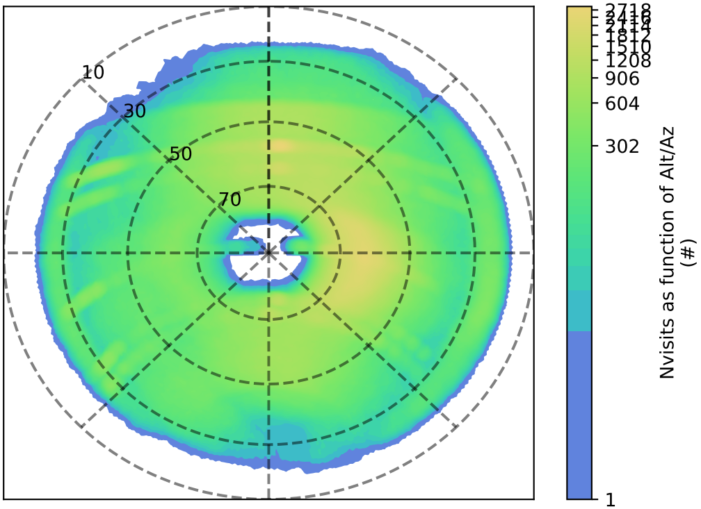
roll_3_v3.4_10yrs i: Nvisits as function of Alt/Az
