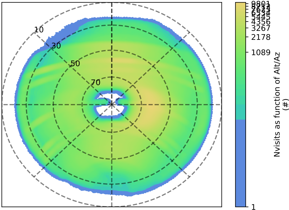
roll_3_v3.4_10yrs : Nvisits as function of Alt/Az
