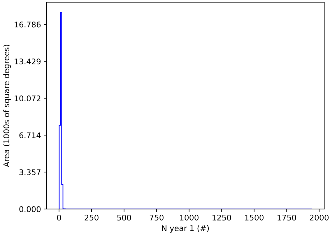
roll_3_v3.4_10yrs z and night < 365: N year 1
