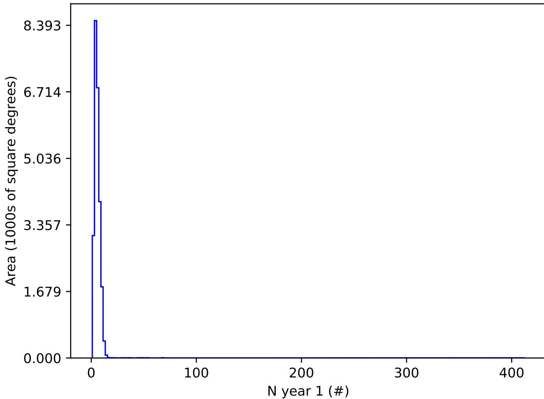
roll_3_v3.4_10yrs u and night < 365: N year 1
