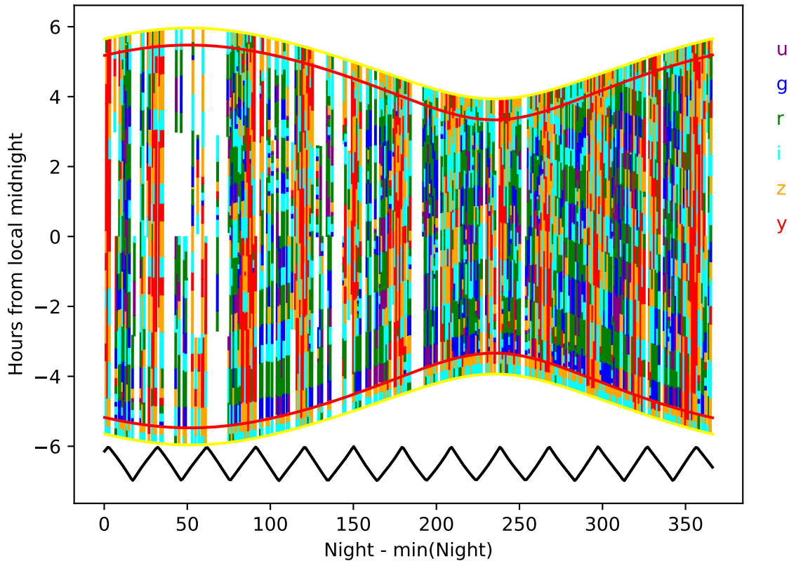
roll_3_v3.4_10yrs year 9-10: Hourglass
