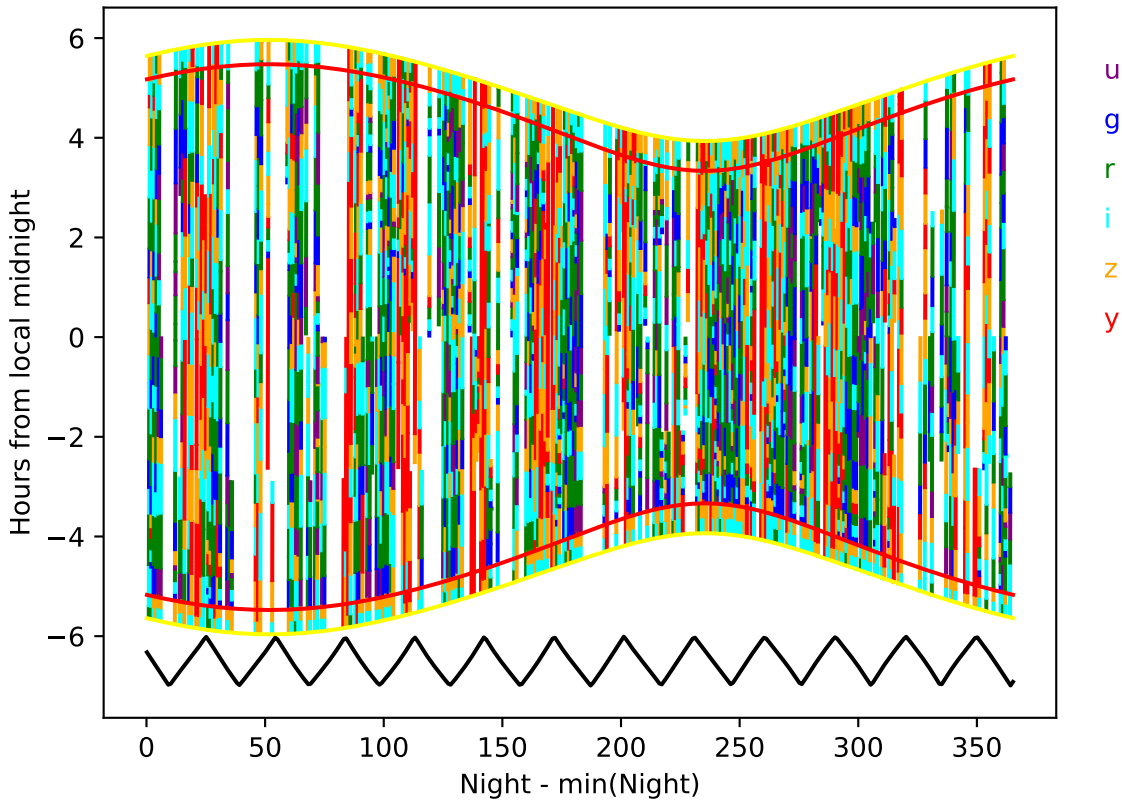
roll_3_v3.4_10yrs year 7-8: Hourglass
