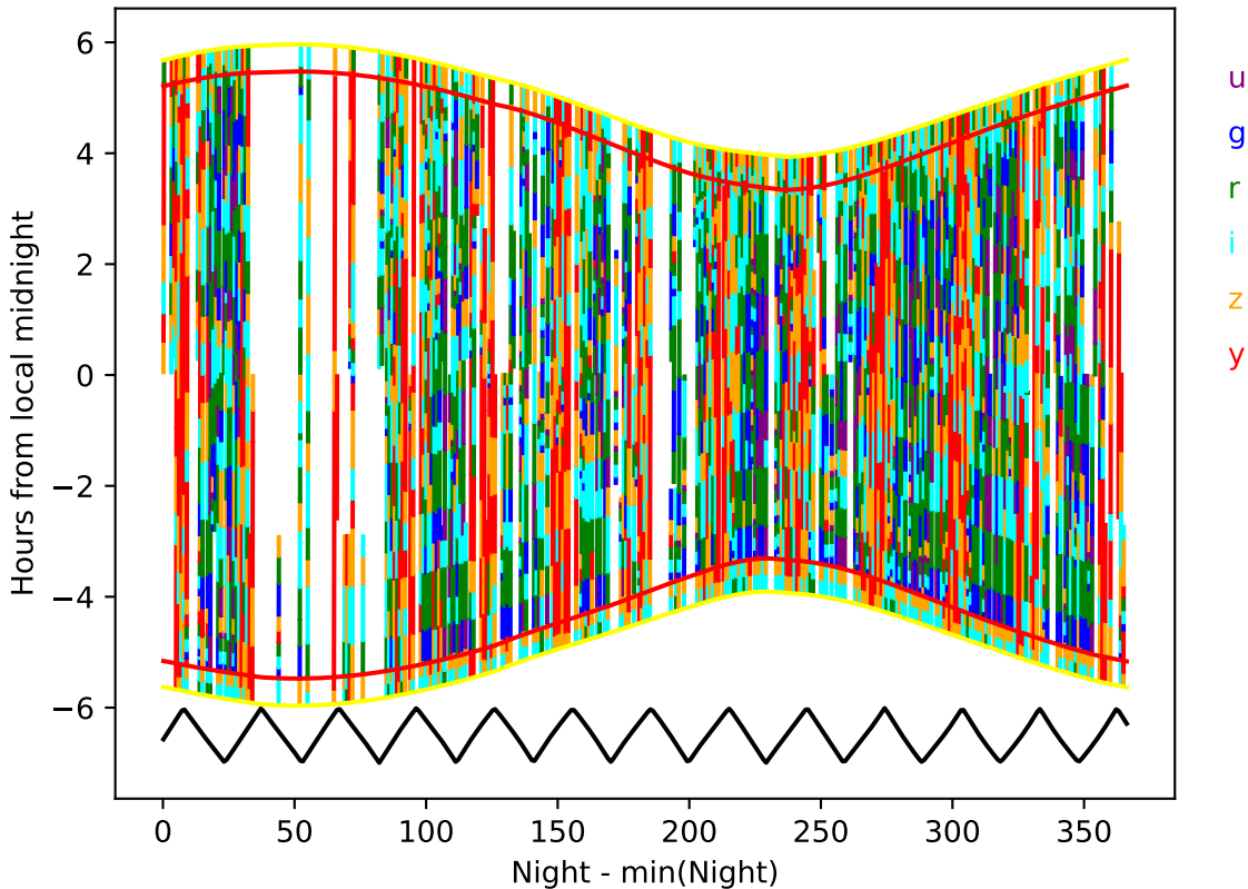
roll_3_v3.4_10yrs year 3-4: Hourglass
