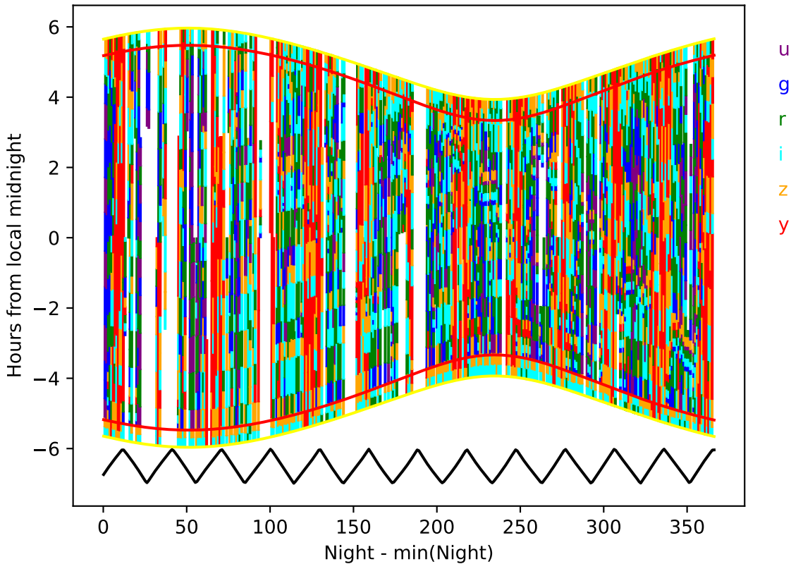
roll_3_v3.4_10yrs year 0-1: Hourglass
