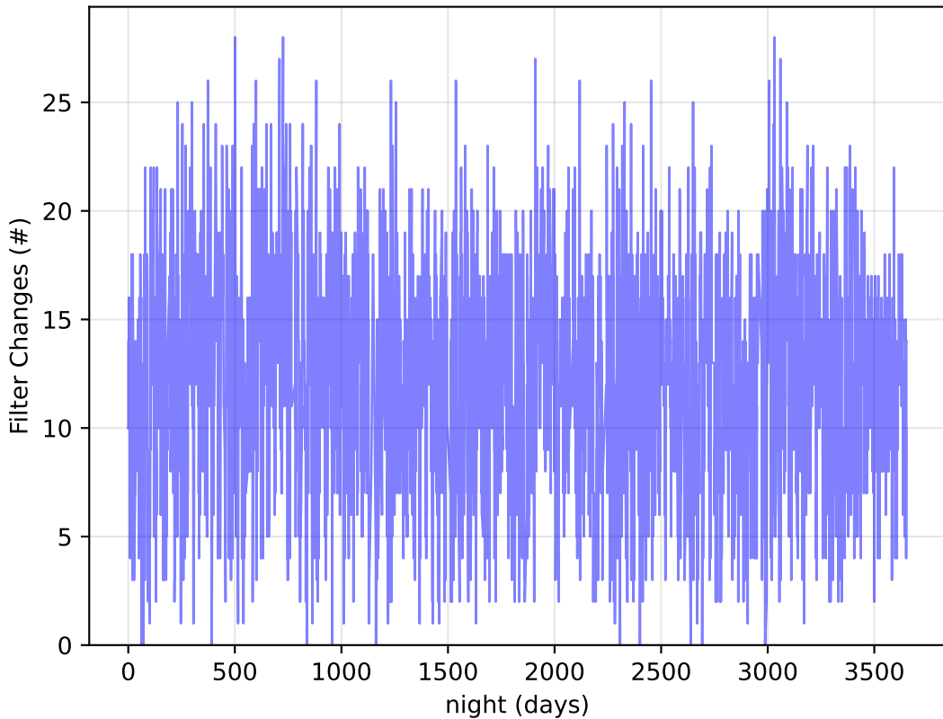
roll_3_v3.4_10yrs : Filter Changes
