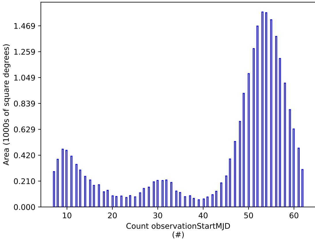
roll_3_v3.4_10yrs u: Count observationStartMJD
