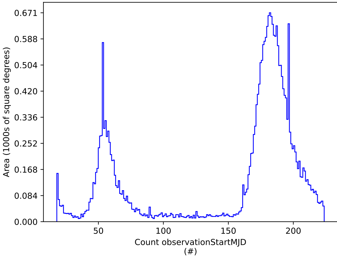
roll_3_v3.4_10yrs r: Count observationStartMJD
