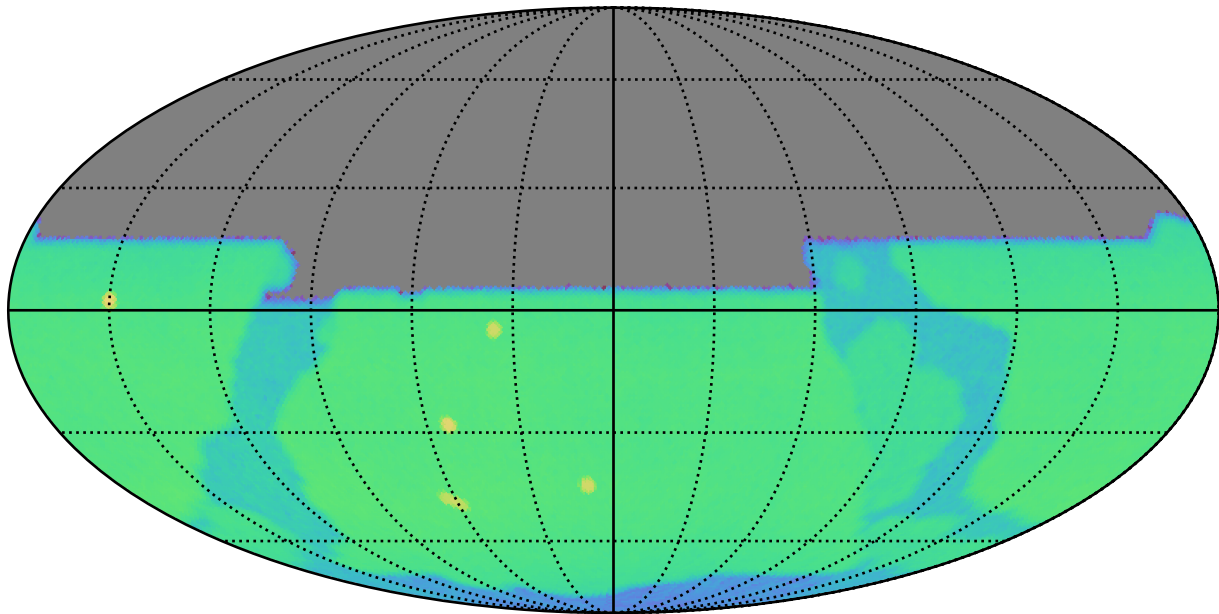
roll_3_v3.4_10yrs y: CoaddM5
