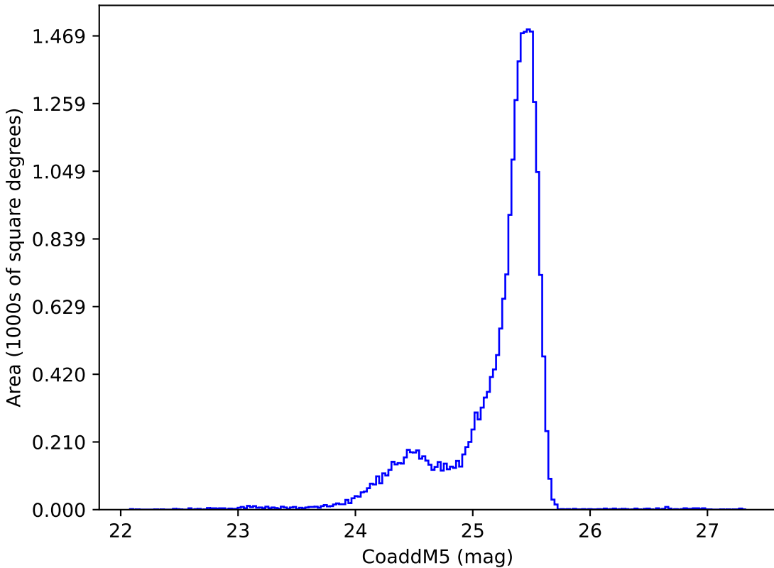
roll_3_v3.4_10yrs u: CoaddM5
