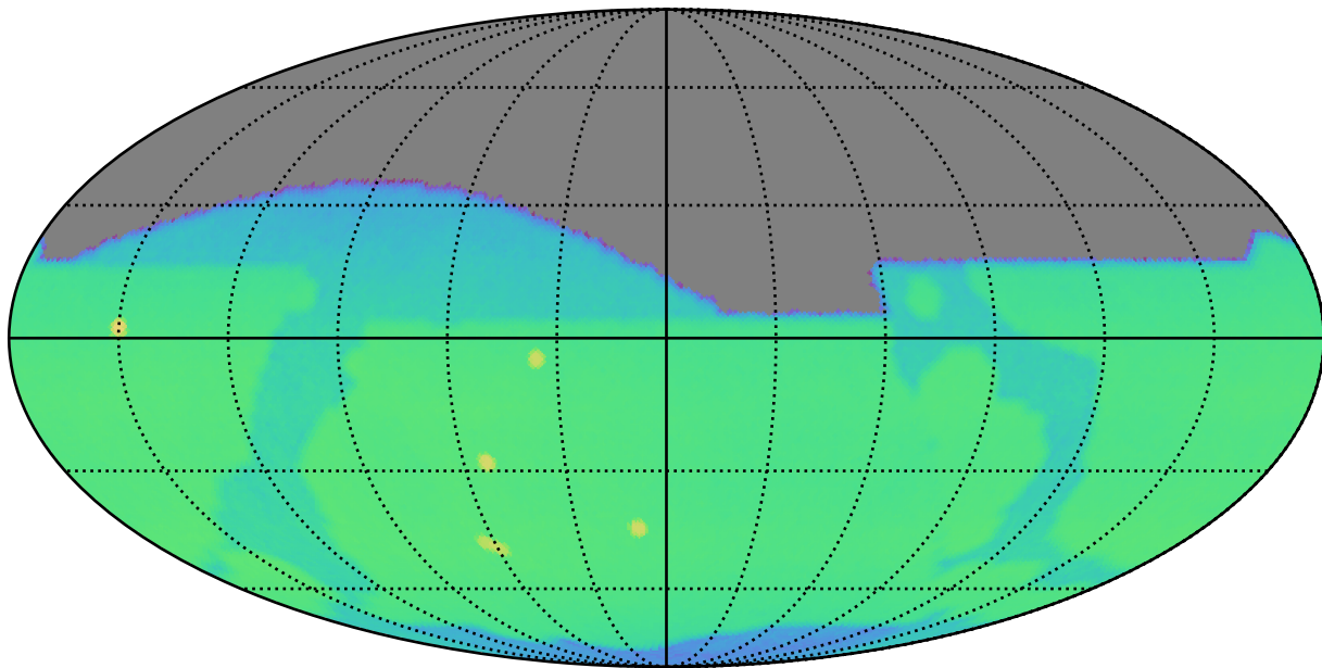
roll_3_v3.4_10yrs r: CoaddM5
