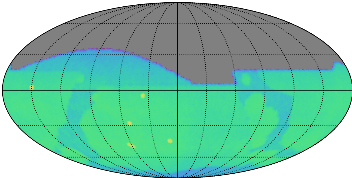
roll_3_v3.4_10yrs g: CoaddM5
