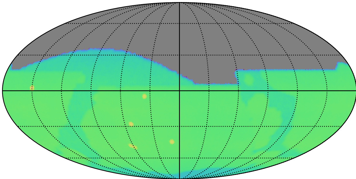
roll_3_v3.4_10yrs : CoaddM5
