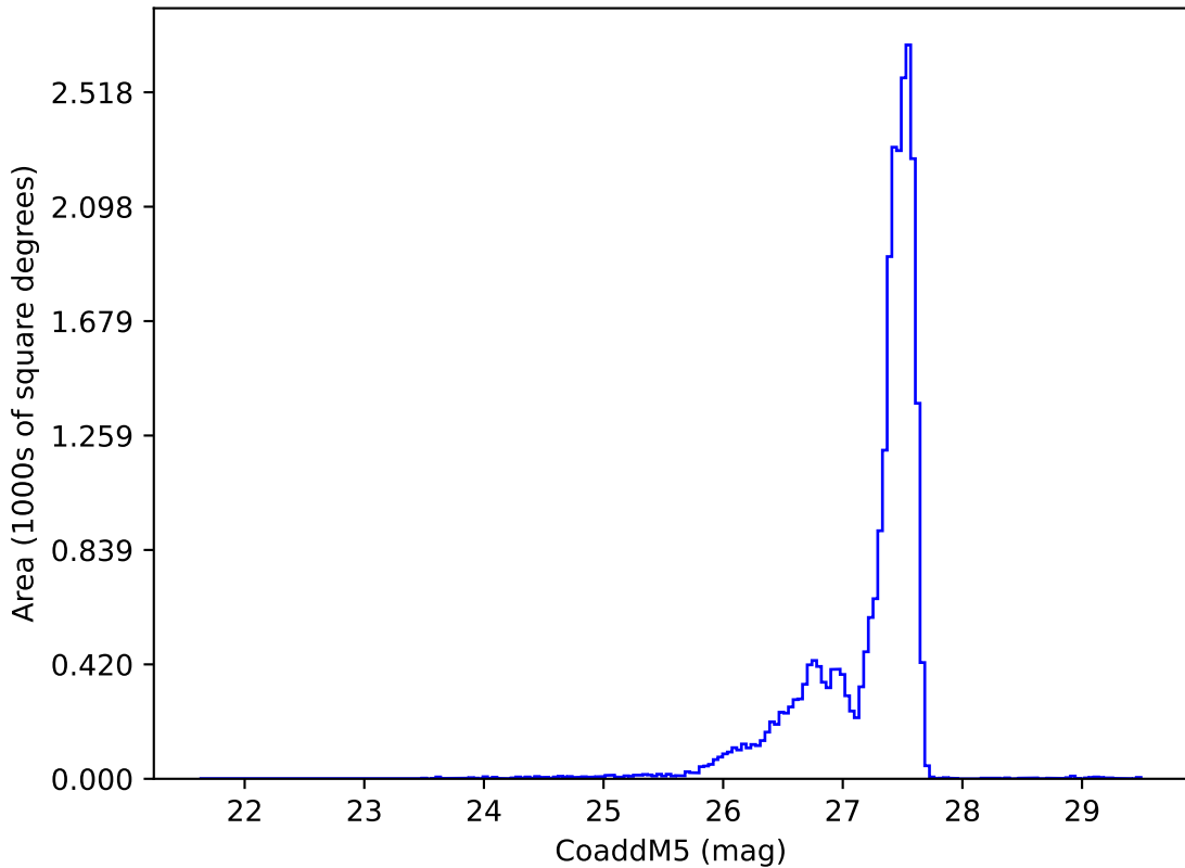
roll_3_v3.4_10yrs : CoaddM5
