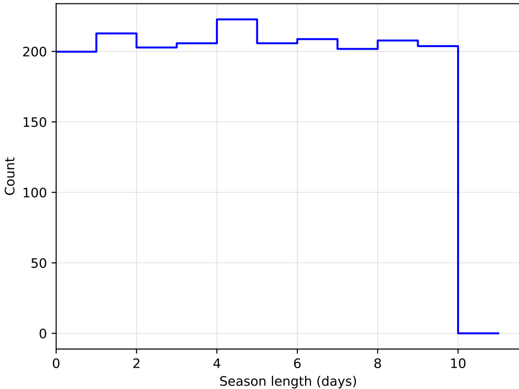
roll_3_v3.4_10yrs DD:XMM_LSS all bands: SeasonLength
