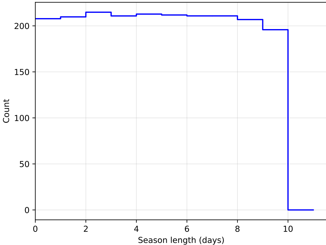
roll_3_v3.4_10yrs DD:EDFS all bands: SeasonLength
