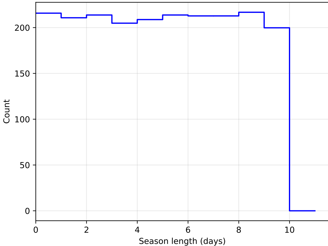
roll_3_v3.4_10yrs DD:ECDFS all bands: SeasonLength
