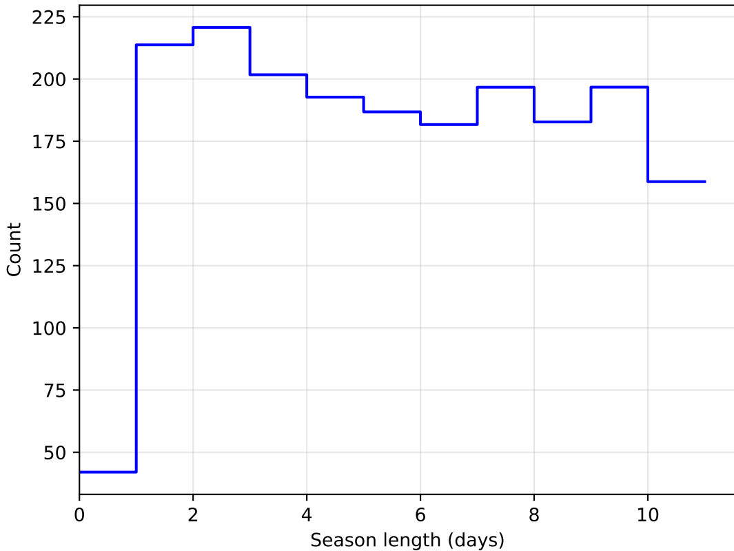
roll_3_v3.4_10yrs DD: COSMOS all bands: SeasonLength
