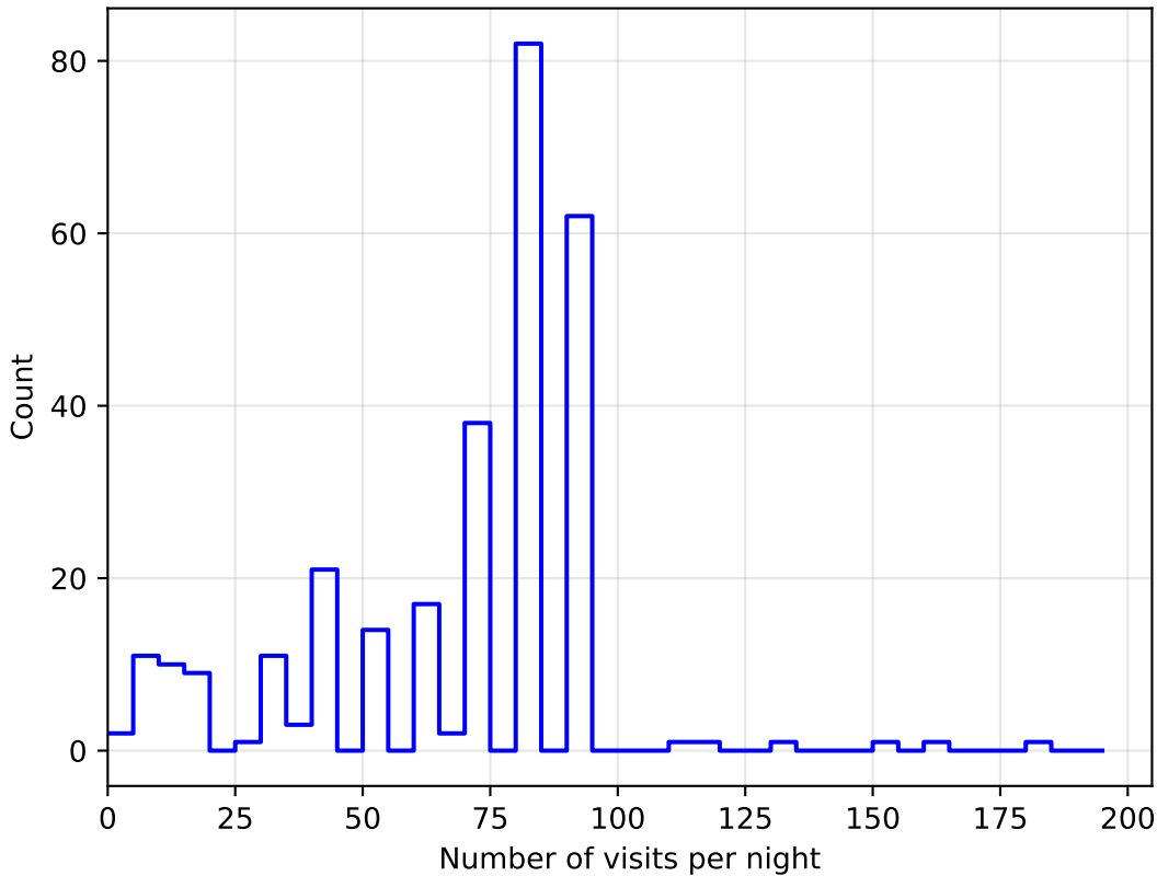
roll_3_v3.4_10yrs all bands: DD:XMM_LSS NVisitsPerNight
