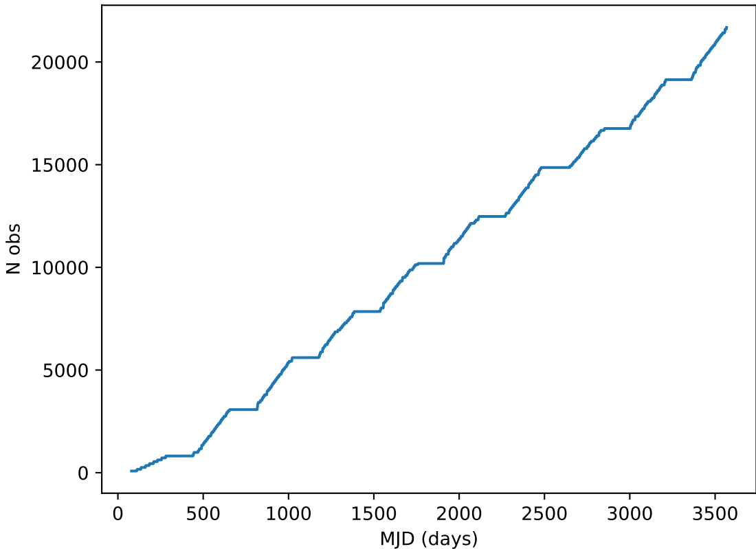
roll_3_v3.4_10yrs all bands: DD:XMM_LSS Cumulative NVisits
