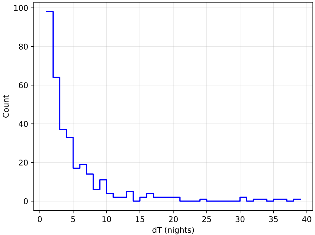
roll_3_v3.4_10yrs all bands: DD:WFD Delta Nights Histogram
