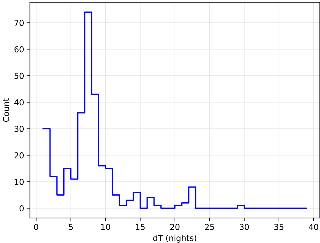
roll_3_v3.4_10yrs all bands: DD:EDFS Delta Nights Histogram
