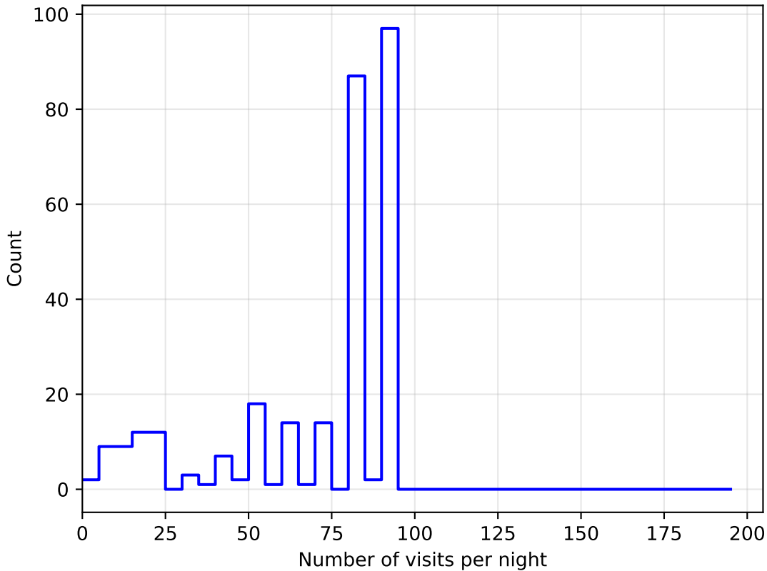
roll_3_v3.4_10yrs all bands: DD:ECDFS NVisitsPerNight
