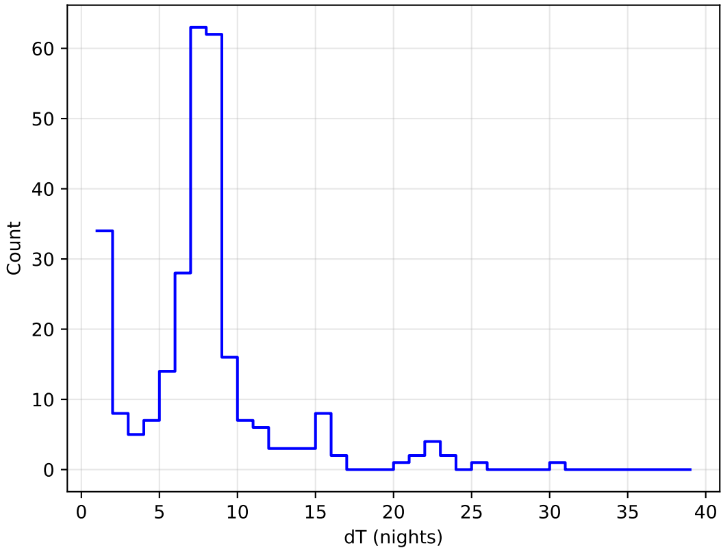
roll_3_v3.4_10yrs all bands: DD:ECDFS Delta Nights Histogram
