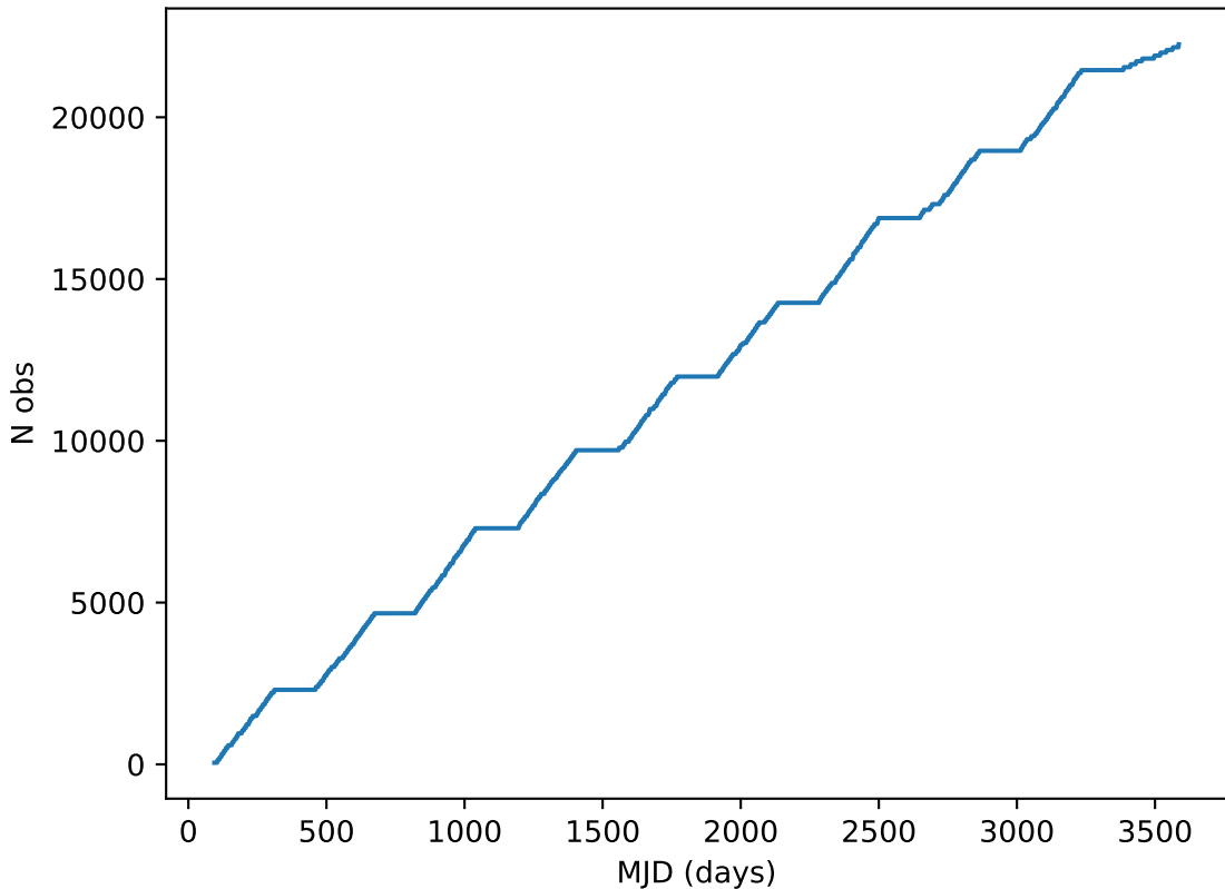
roll_3_v3.4_10yrs all bands: DD:ECDFS Cumulative NVisits
