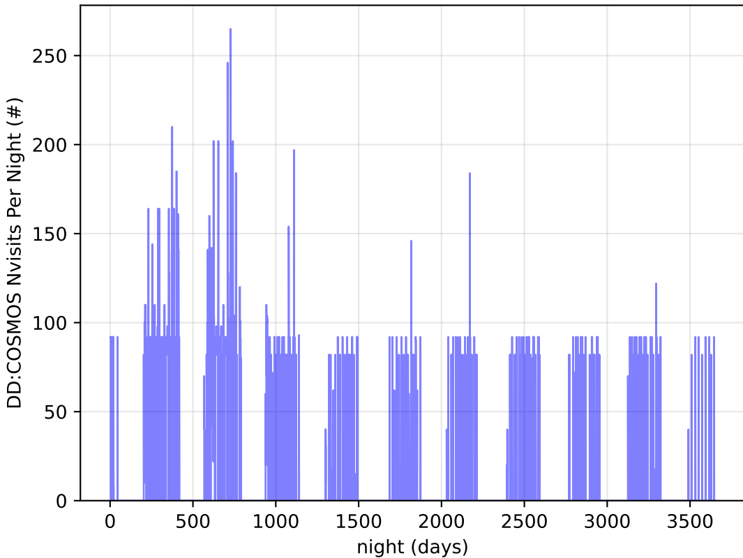
roll_3_v3.4_10yrs all bands: DD: COSMOS Nvisits Per Night
