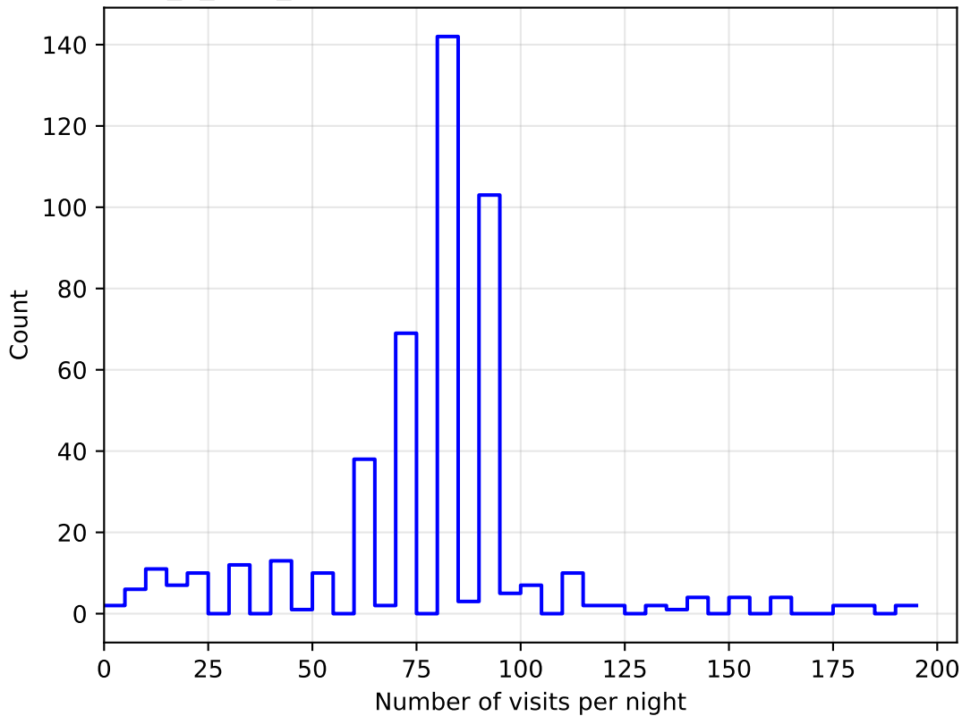
roll_3_v3.4_10yrs all bands: DD: COSMOS NVisitsPerNight
