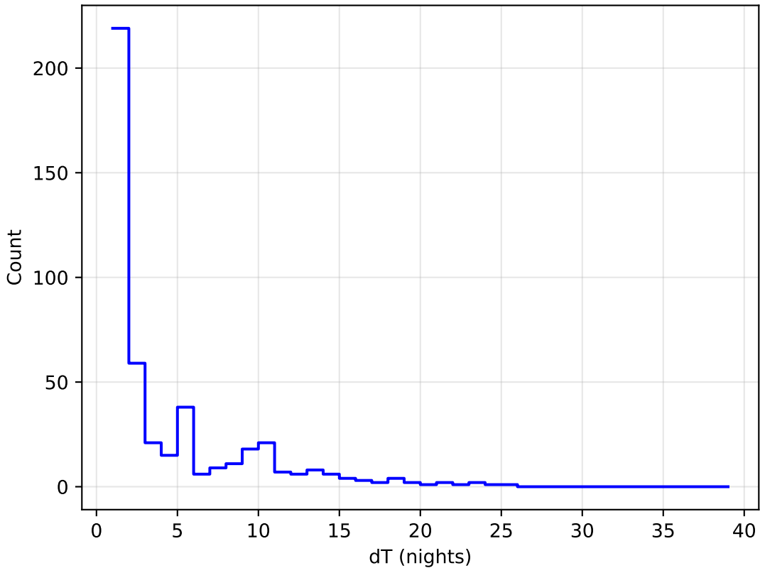
roll_3_v3.4_10yrs all bands: DD:COSMOS Delta Nights Histogram
