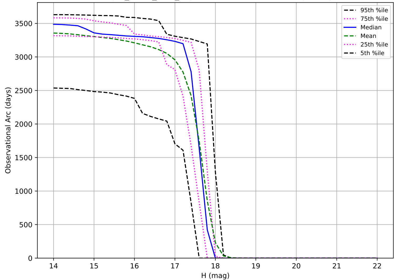
reweight_plane_v3.3_10yrs: Observational Arc Length Trojan
