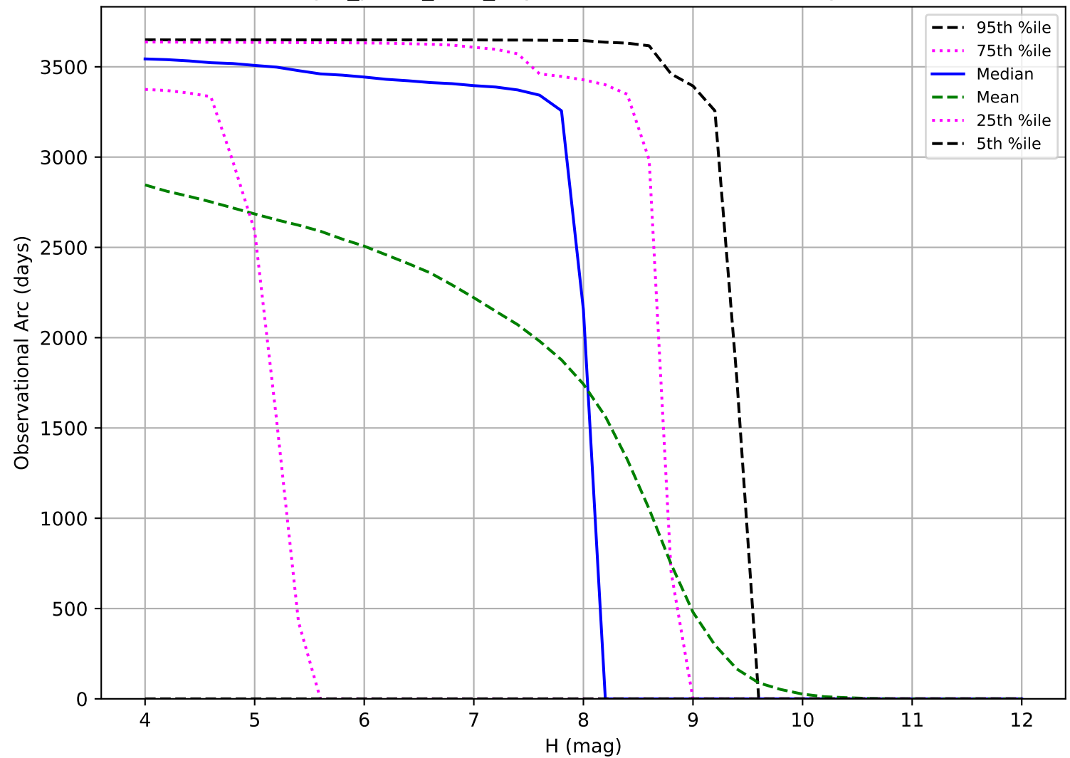
reweight_plane_v3.3_10yrs: Observational Arc Length TNO
