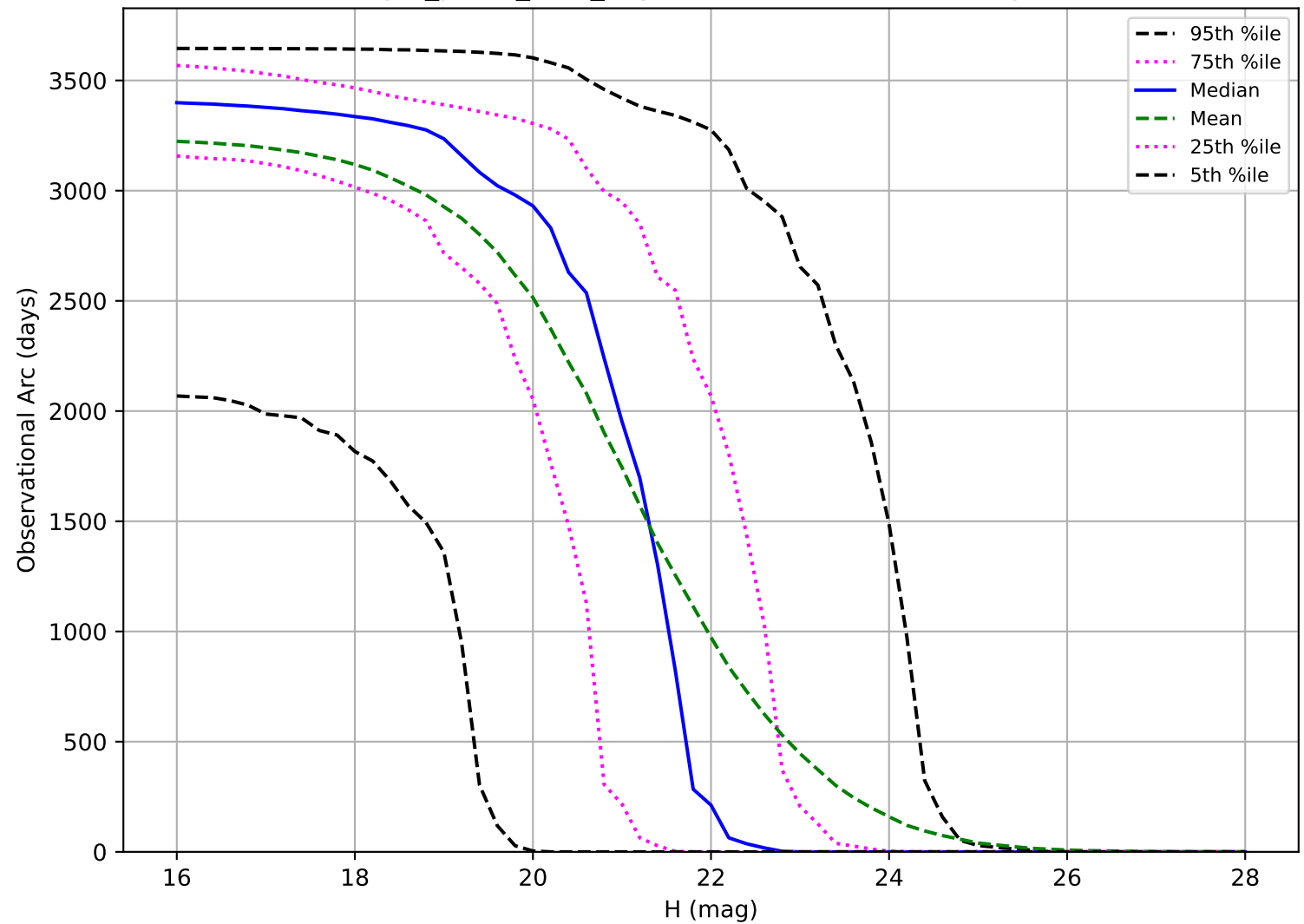
reweight_plane_v3.3_10yrs: Observational Arc Length PHA
