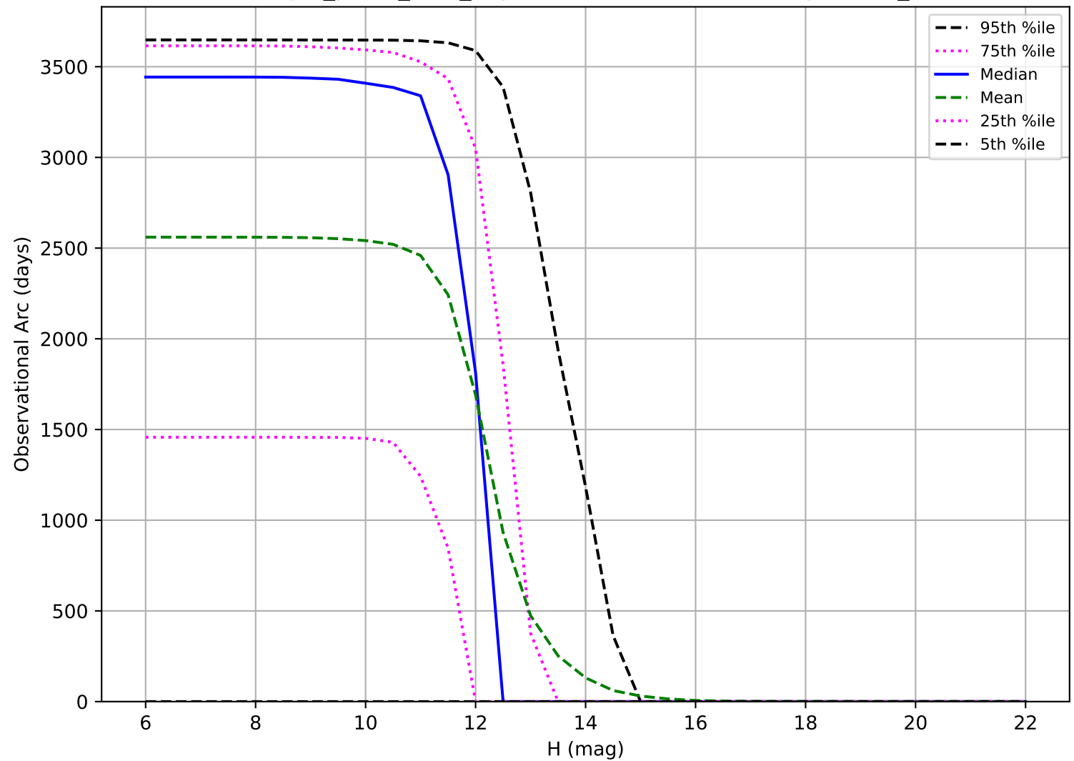
reweight_plane_v3.3_10yrs: Observational Arc Length OCC_r20
