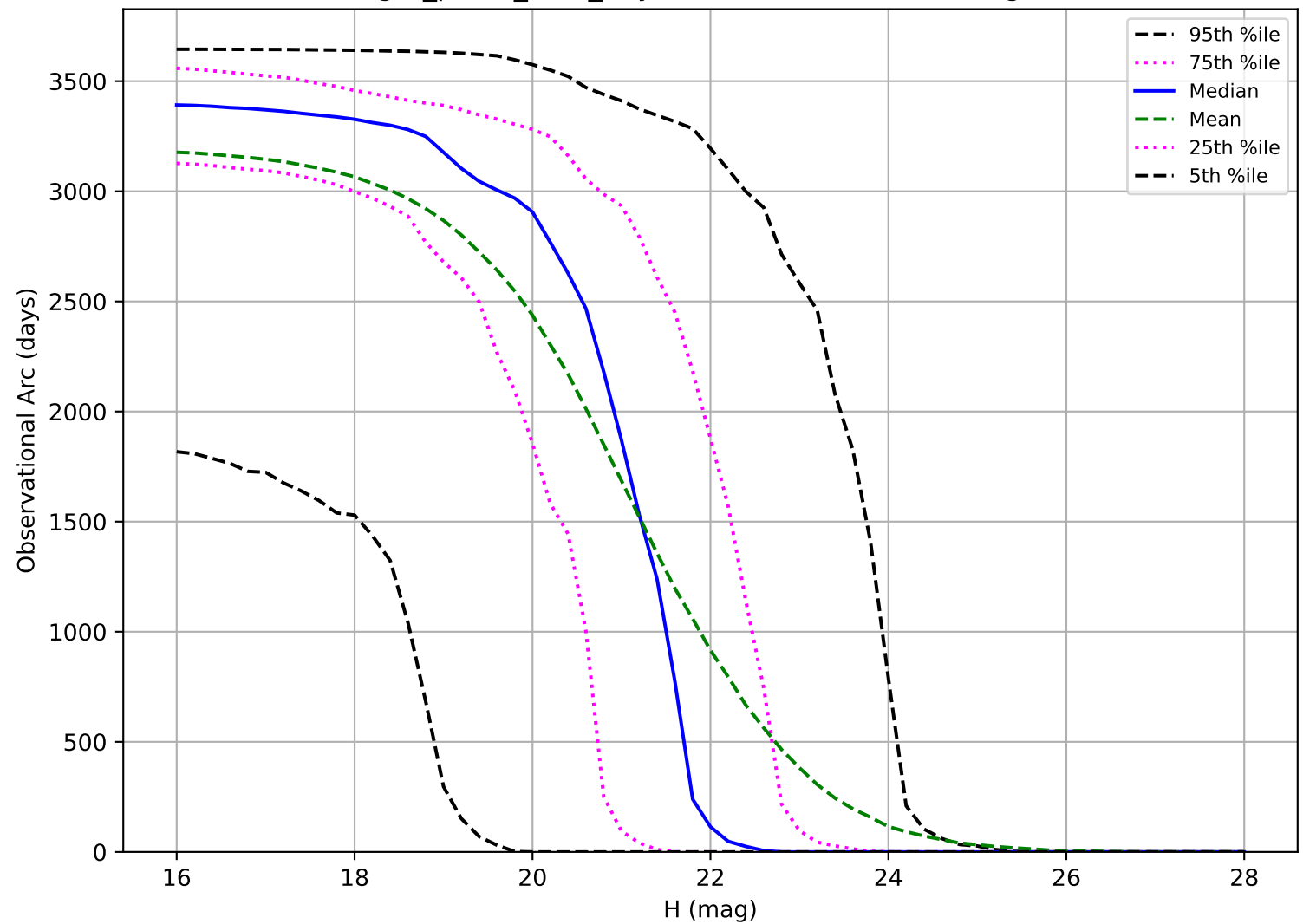
reweight_plane_v3.3_10yrs: Observational Arc Length NEO
