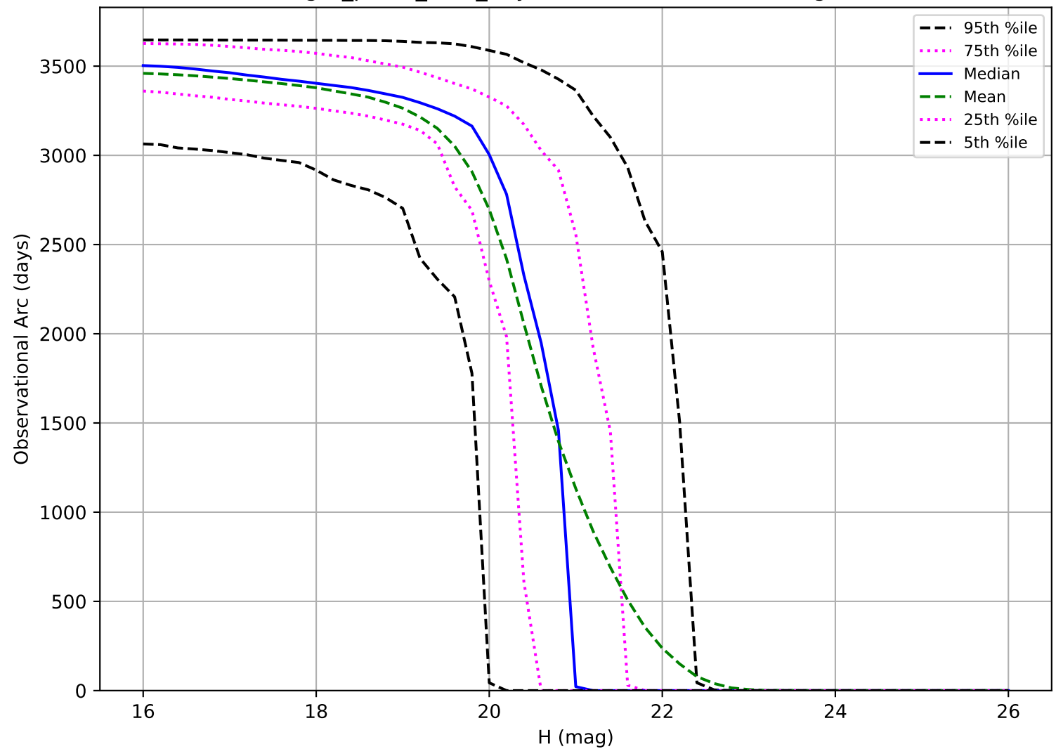
reweight_plane_v3.3_10yrs: Observational Arc Length MBA
