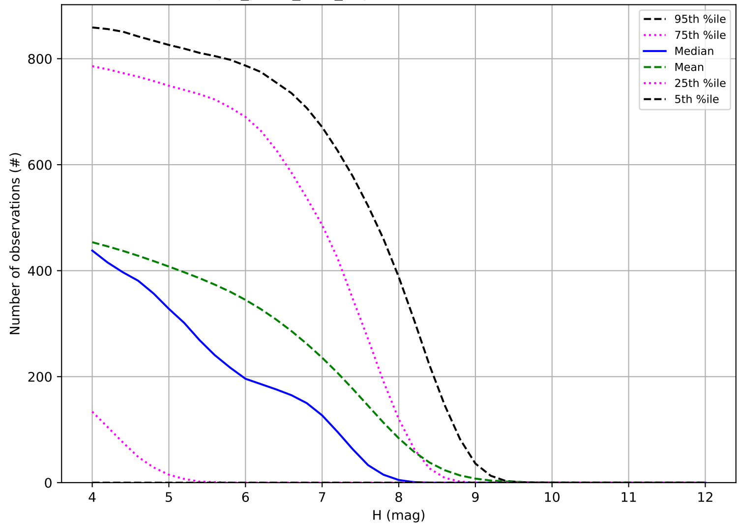
reweight_plane_v3.3_10yrs: Number of observations TNO
