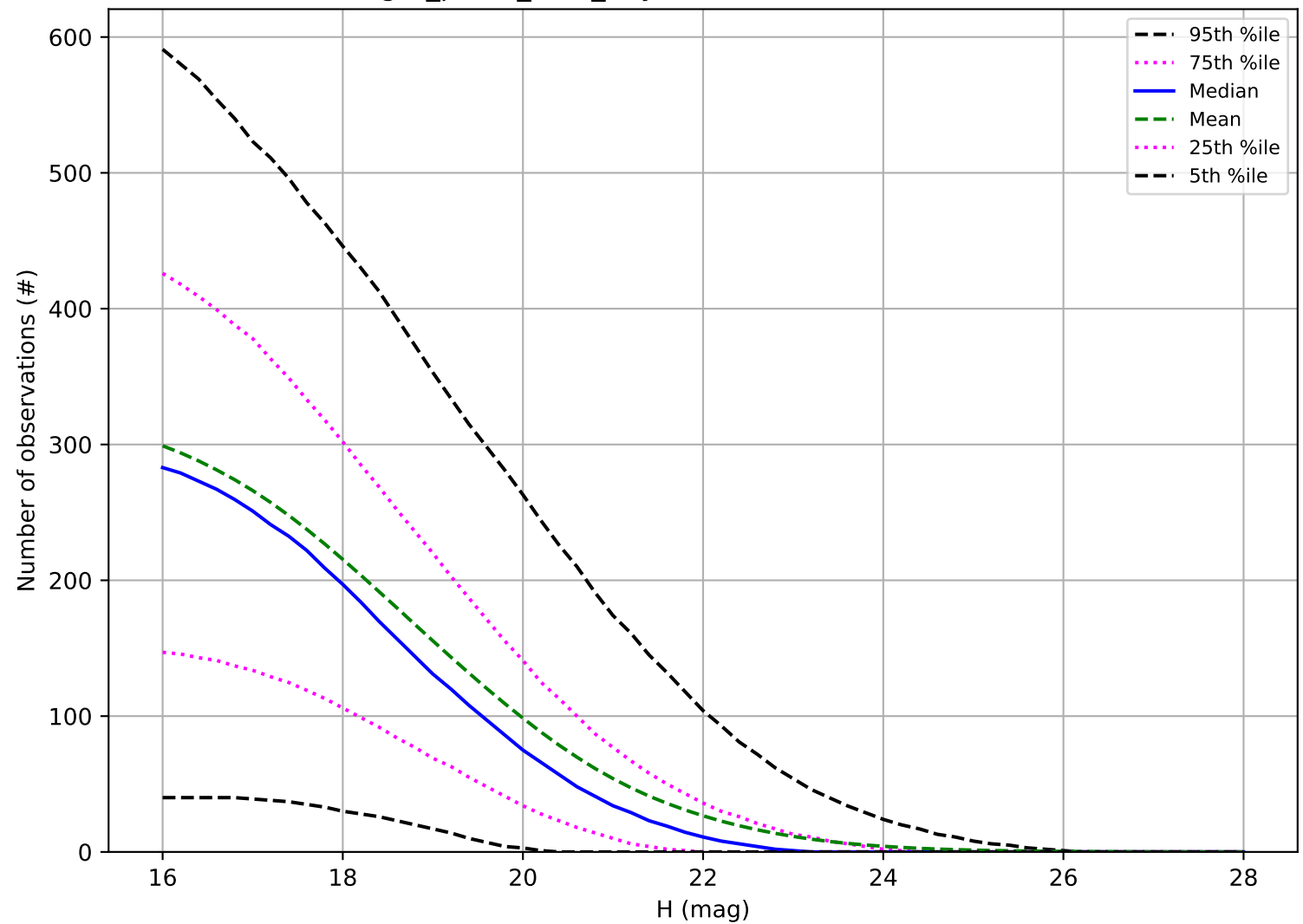
reweight_plane_v3.3_10yrs: Number of observations PHA
