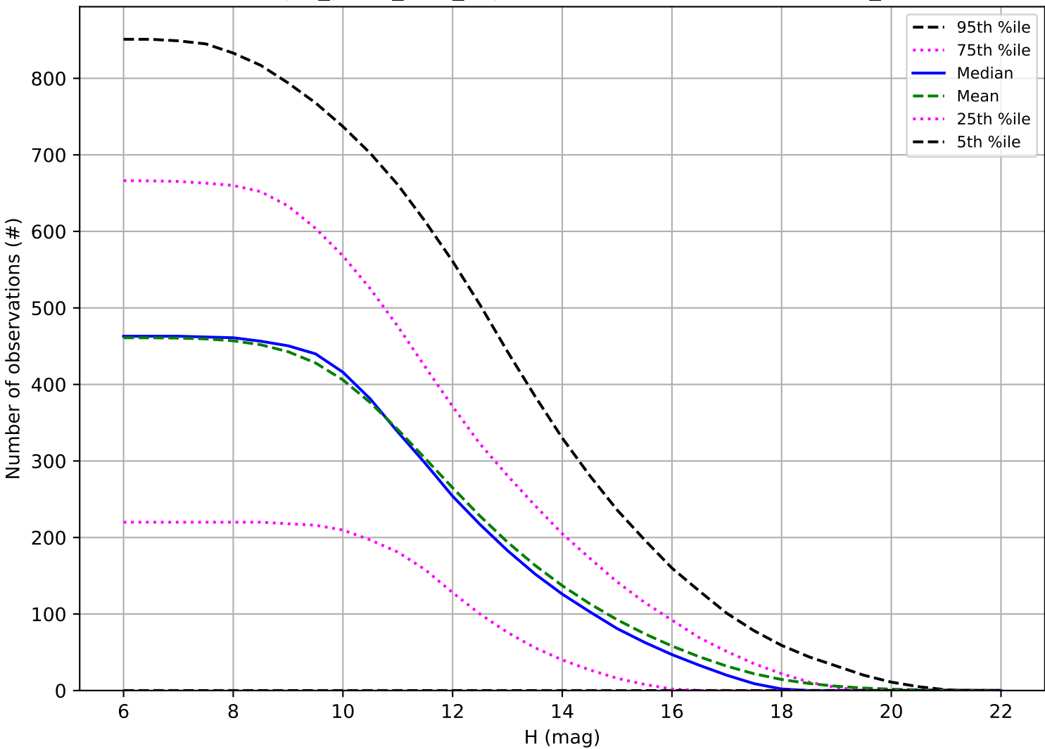
reweight_plane_v3.3_10yrs: Number of observations OCC_r5
